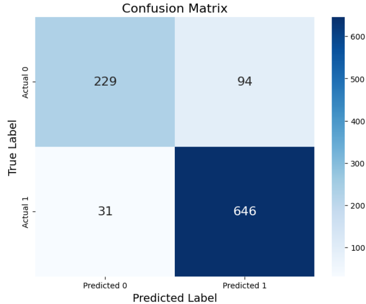
Figure 1 BERT-ita (no additional features) confusion matrix on the test set
